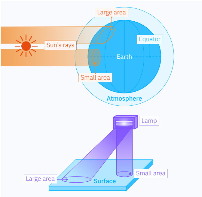
FIGURE 2.3. Illustration of angular dependence. Source: Peter Halasz on Wikipedia, licensed under CC BY-SA 2.5 16 .
