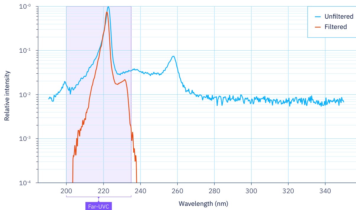
FIGURE 8.4. Comparison of a filtered and unfiltered KrCl* spectrum, logarithmic scale. Data from OSLUV Assays 9 .
