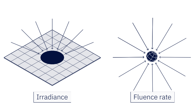
FIGURE 2.2. Irradiance versus fluence rate . Source: Ultraviolet Germicidal Irradiation Handbook 5 .
