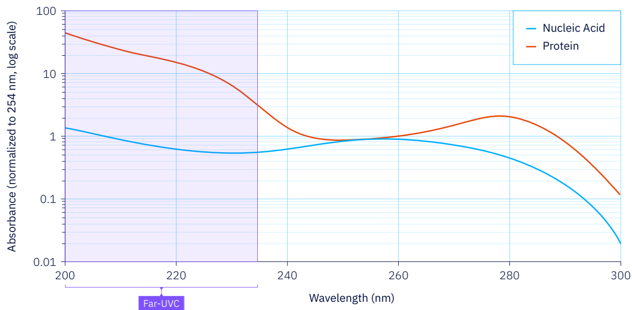
FIGURE 2.5. Excerpted from IUVA, 2021 1 ; original sources Setlow and Doyle, 1957 13 and Voet et al., 1963 14 . Nucleic acid and protein absorbance spectra by wavelength, normalized to 254 nm on a logarithmic vertical scale.
