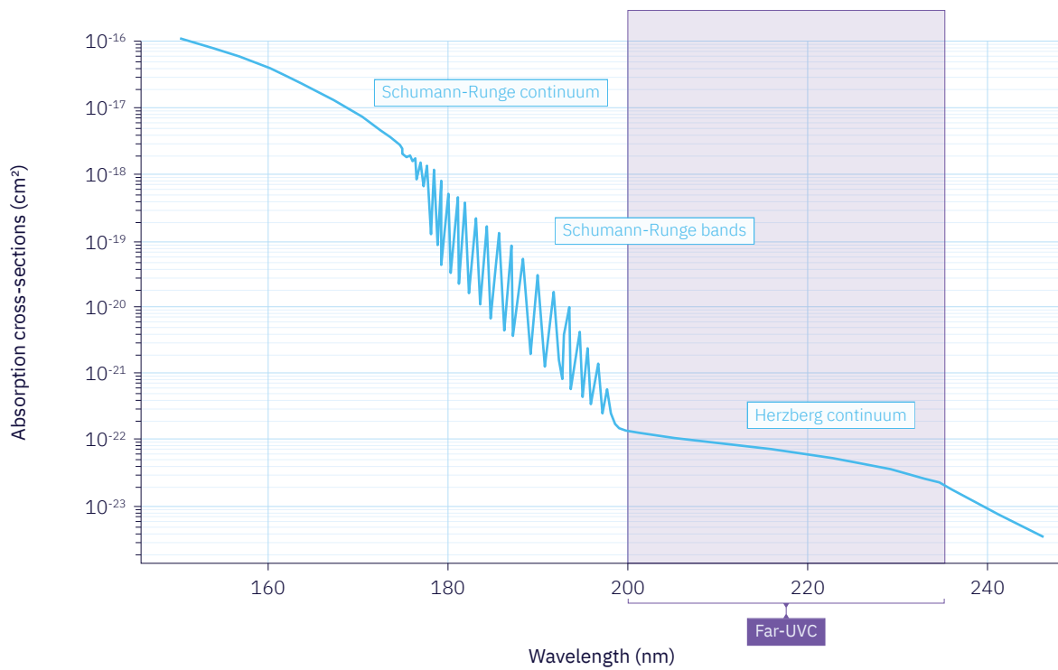
FIGURE 6.1. Excerpted from Watanabe, Inn and Zelickoff, 1953 1 . Absorption cross-section of O 2 (log scale).
