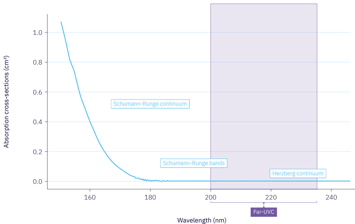
FIGURE 6.2. Excerpted from Watanabe, Inn and Zelickoff, 1953 1 . Absorption cross-section of O 2 (linear scale).
