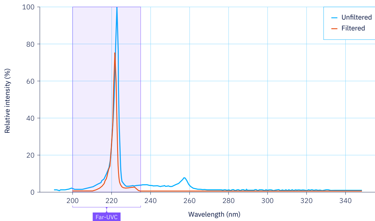
FIGURE 8.5. Comparison of a filtered and unfiltered KrCl* spectrum, linear scale. Data from OSLUV Assays 9 .
