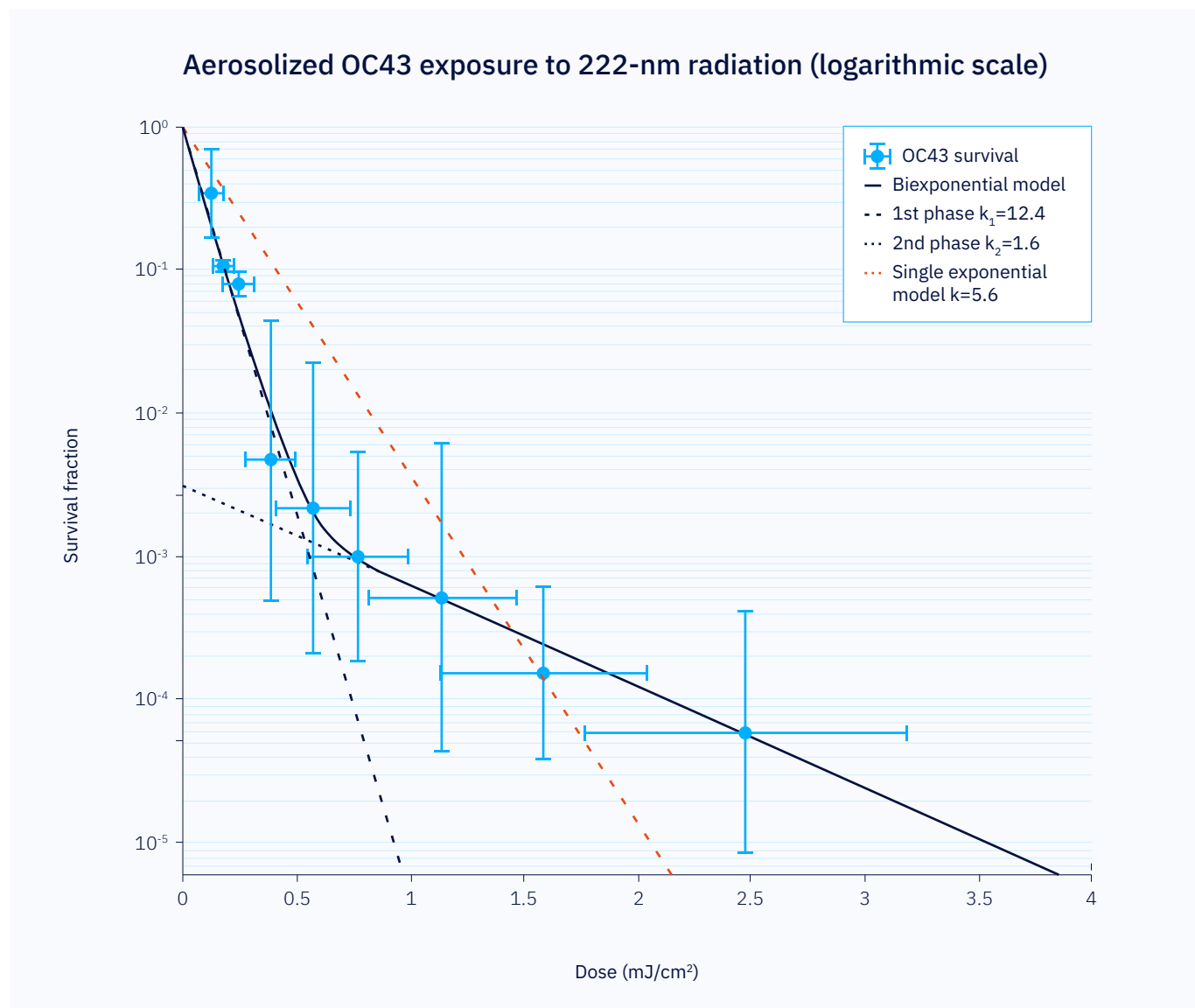
FIGURE 3.1. Excerpted from Welch, 2022 34 . Survival fraction of coronavirus OC43 exposed to 222-nm radiation fitted with the two-phase decay model. The circle markers represent the mean survival values for a given mean exposure dose. The x-error bars show the standard deviation of the doses for the 1600 particles in the simulation, and the y-error bars show the standard deviation of the experimental repeats of survival fraction. The two-phase decay model fit to the data is included on the graph (solid line), as well as lines representing the decay of the first and second stages separately (dashed and dotted lines, respectively). The single exponential model fit to the same data is included for comparison.
