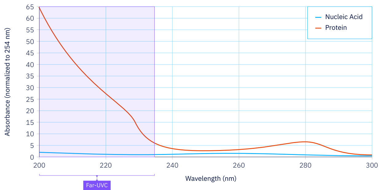
FIGURE 2.6. Excerpted from IUVA, 2021 1 ; original sources Setlow and Doyle, 1957 13 and Voet et al., 1963 14 . Nucleic acid and protein absorbance spectra by wavelength, normalized to 254 nm on a linear vertical scale.
