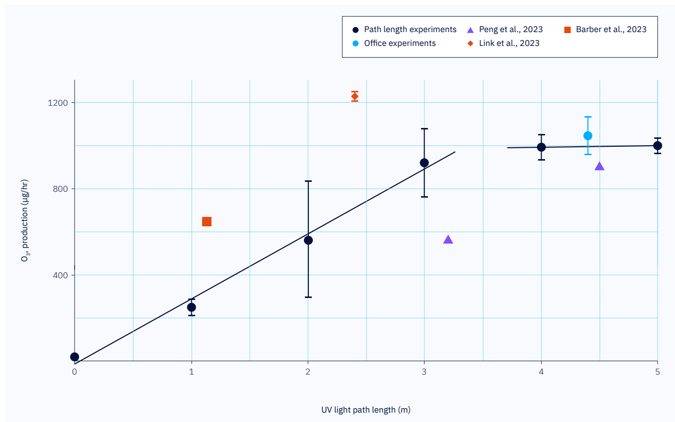
FIGURE 6.4. Excerpted from Sørensen et al., 2024 10 . Correlation between O 3 production (µg/hr) and UV light path length (m) according to the Sørensen et al. study (circles) and the pre-existing literature (triangles, square, and diamond). The equation displayed gives the linear correlation from 0 to 3 m, while the error bars indicate the standard deviations. Pressure corrections have been made for the results from Peng et al. to account for the reduced ambient pressure in Boulder where the experiments were carried out.
